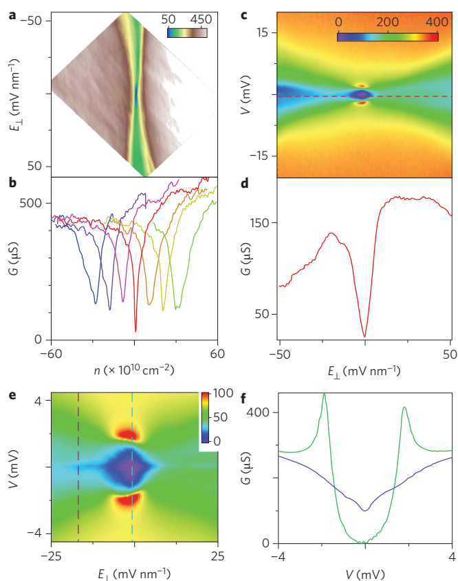
Figure 2 | Transport data at B = 0 and T = 300 mK. a,b , G(n, E_{\perp}) and line traces G(n) at E_{\perp} = -37.5, -25, -12.5, 0, 12.5, 25 and 37.5 \text{mV nm}^{-1} , respectively (left to right). The line traces are laterally offset for clarity and the colour scale is in units of conductance, \mu\text{S} . c,d , Large-range G(V, E_{\perp}) in units of \mu\text{S} and line trace G(E_{\perp}) at n = 0 . e , High-resolution G(V, E_{\perp}) for small bias range at n = 0 . f , Line traces G(V) along the dotted lines in e at E_{\perp} = 0 (purple) and -15 \text{mV nm}^{-1} (green), respectively.
