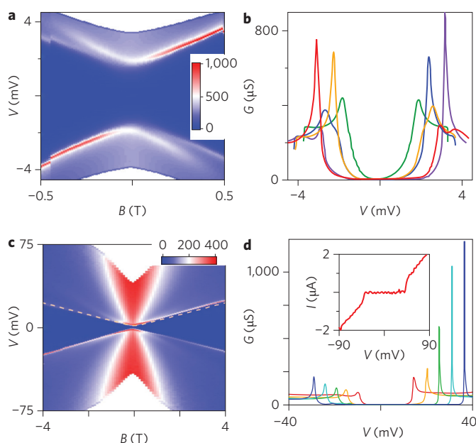
Figure 3 | Transport data in magnetic field at n = 0 and E_{\perp} = 0 .
