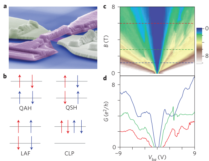
Figure 1 | Device image, proposed gapped states in bilayer graphene and quantum Hall data at 300 mK.
