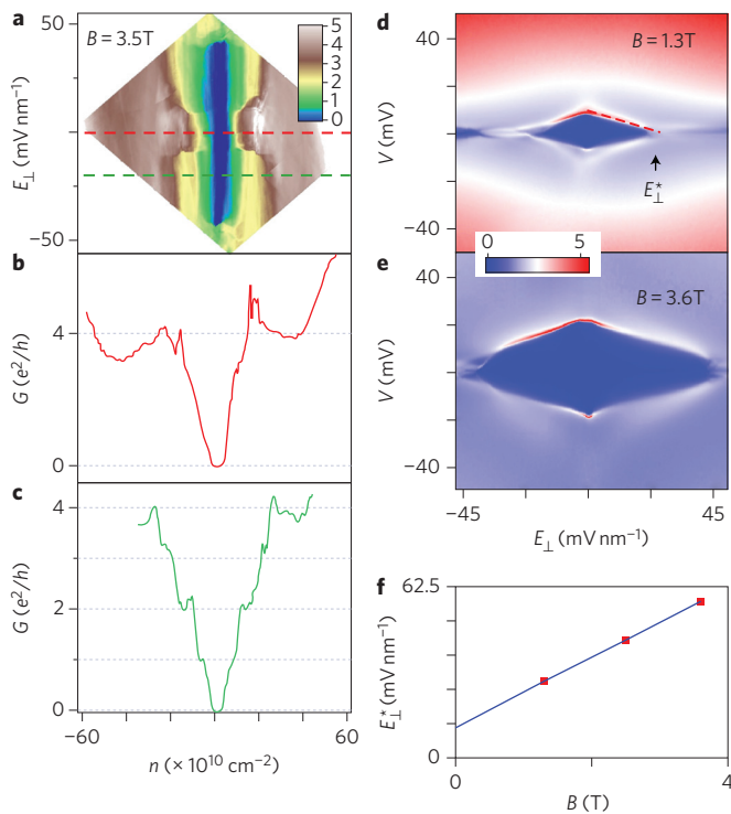
Figure 4 | Transport data at constant B . a , G(n, E) in units of e^2/h at B = 3.5 T. b,c , Line traces G(n) along the dotted lines in a at E_{\perp} = 0 (red) and -20 mV nm ^{-1} (green). d,e , G(V, E) at B = 1.3 T and 3.6 T, respectively. Both colour scales are in conductance units of e^2/h . f , Critical electric field E_{\perp}^* versus B . The blue line is a best fit to data, with a slope of 12.7 mV nm ^{-1} T ^{-1} .
